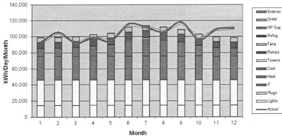
Figure 2 Actual versus predicted electrical energy usage.
