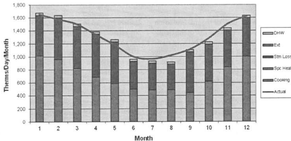
Figure 3 Actual versus predicted natural gas usage.
